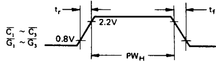
Figure 4 Input Pulse Width "High"
