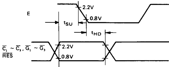
Figure 5 Input Setup and Hold Times
