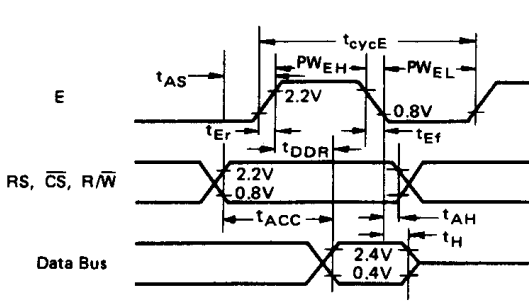
Figure 1 Bus Read Timing (Read Information from PTM)
