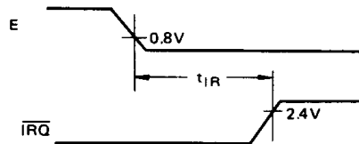
Figure 7 \overline{IRQ} Release Time
