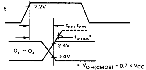
Figure 6 Output Delay
