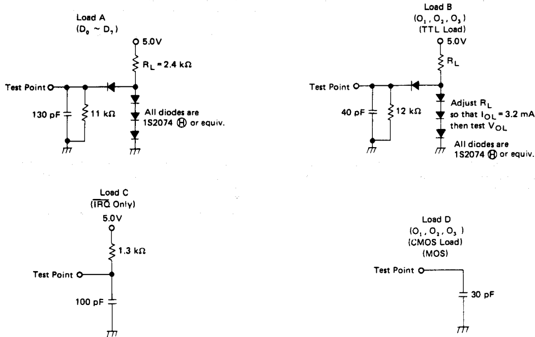
Figure 8 Test Loads
